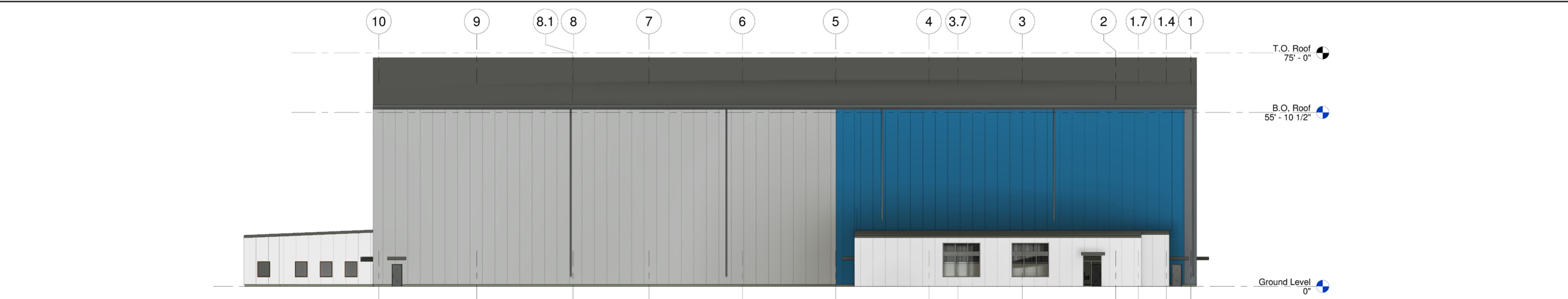
1 West Elevation - Presentation A-000B 1/16" = 1'-0"
