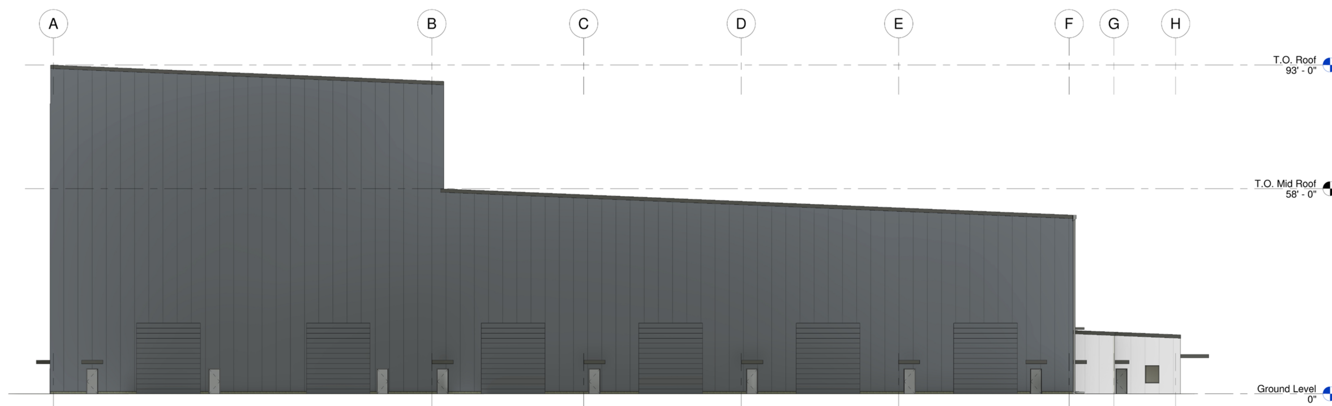
3 North Elevation - Presentation A-000D 1/16" = 1'-0"
