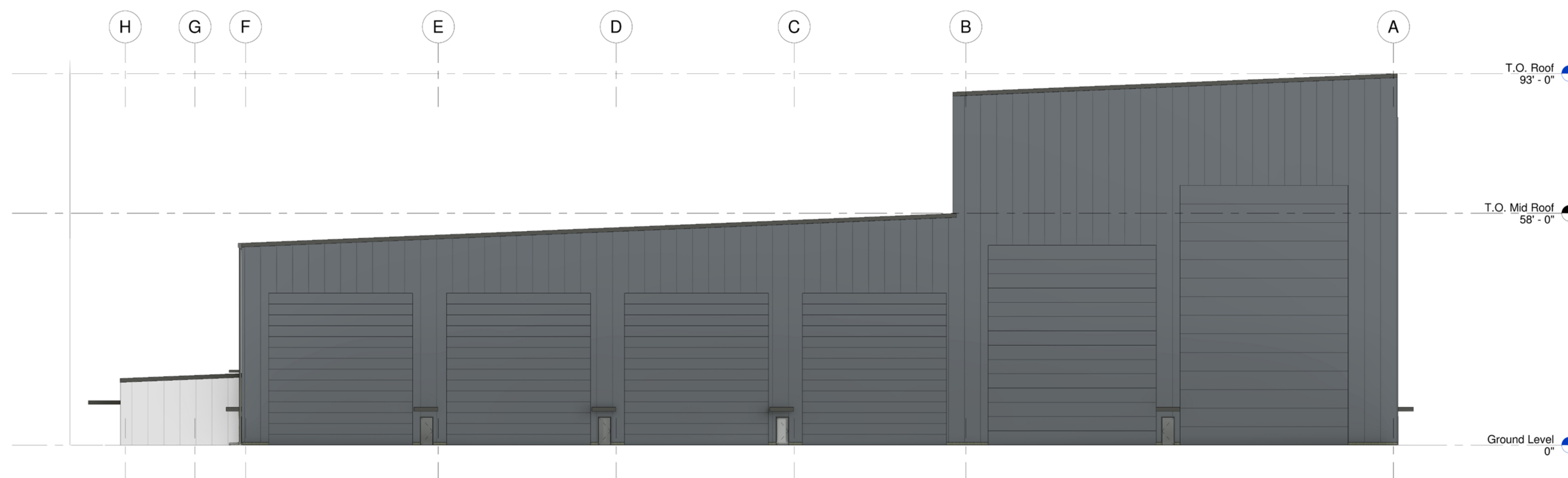
4 South Elevation - Presentation A-000D 1/16" = 1'-0"
